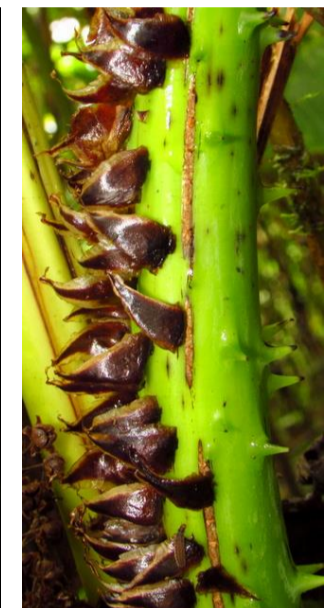
petiole
