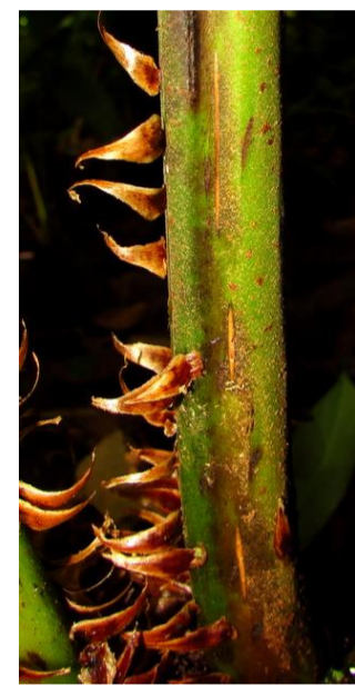
petiole
