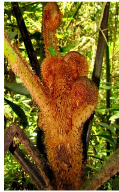
trunk apex
