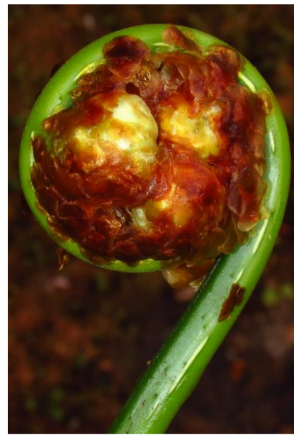
crozier
