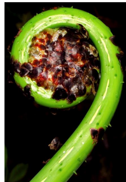
crozier
