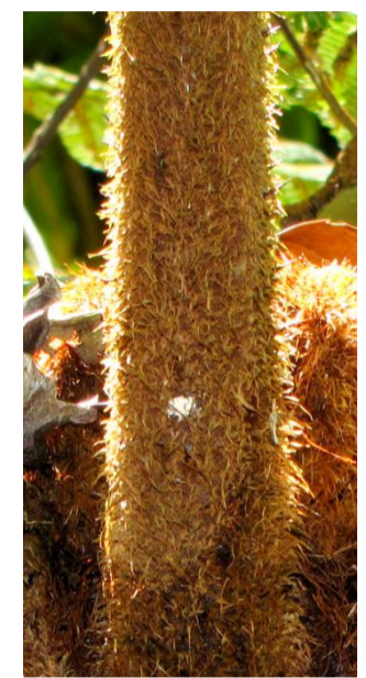
petiole
