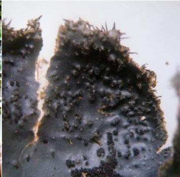
18 Sticta LOBARIACEAE
