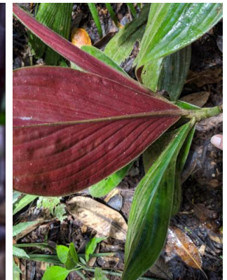
10 C. amazonicus ssp. krukovii
